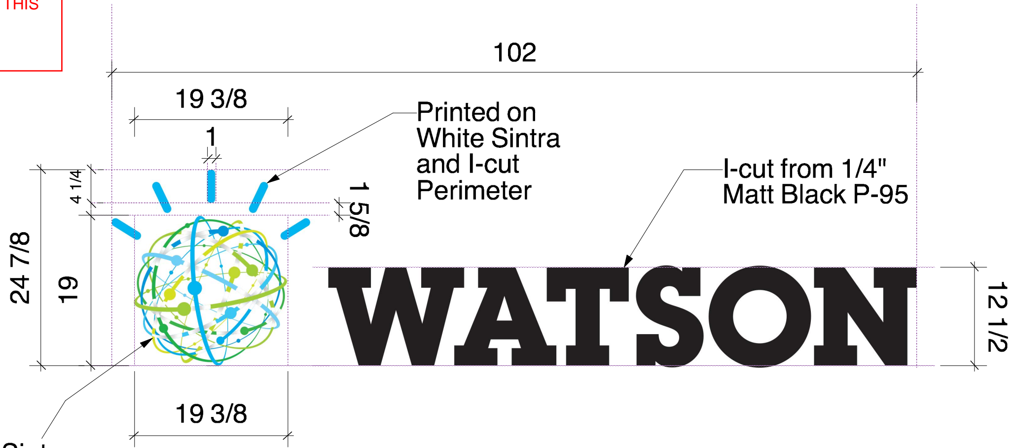
1 Wall: A Horizontal Lock-up Scale: 1" = 1'-0"
