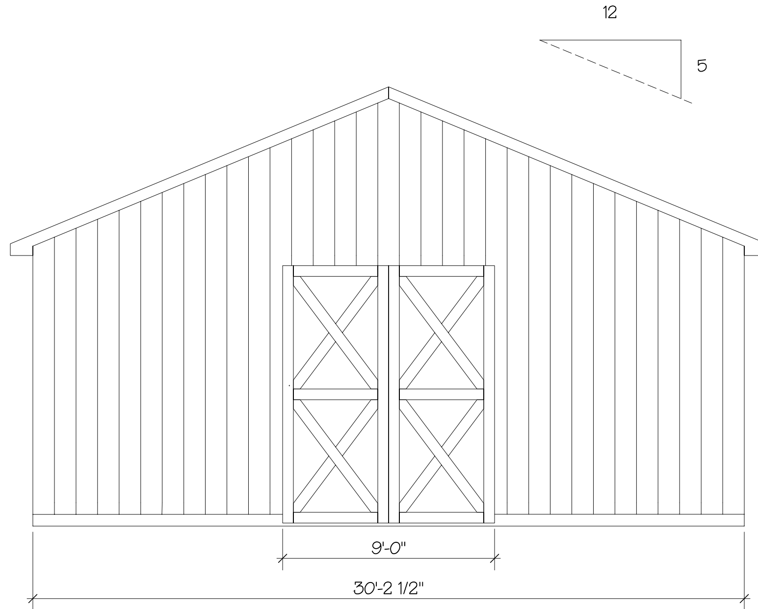
3 Front Elevation Scale: 1/4" = 1'-0"
