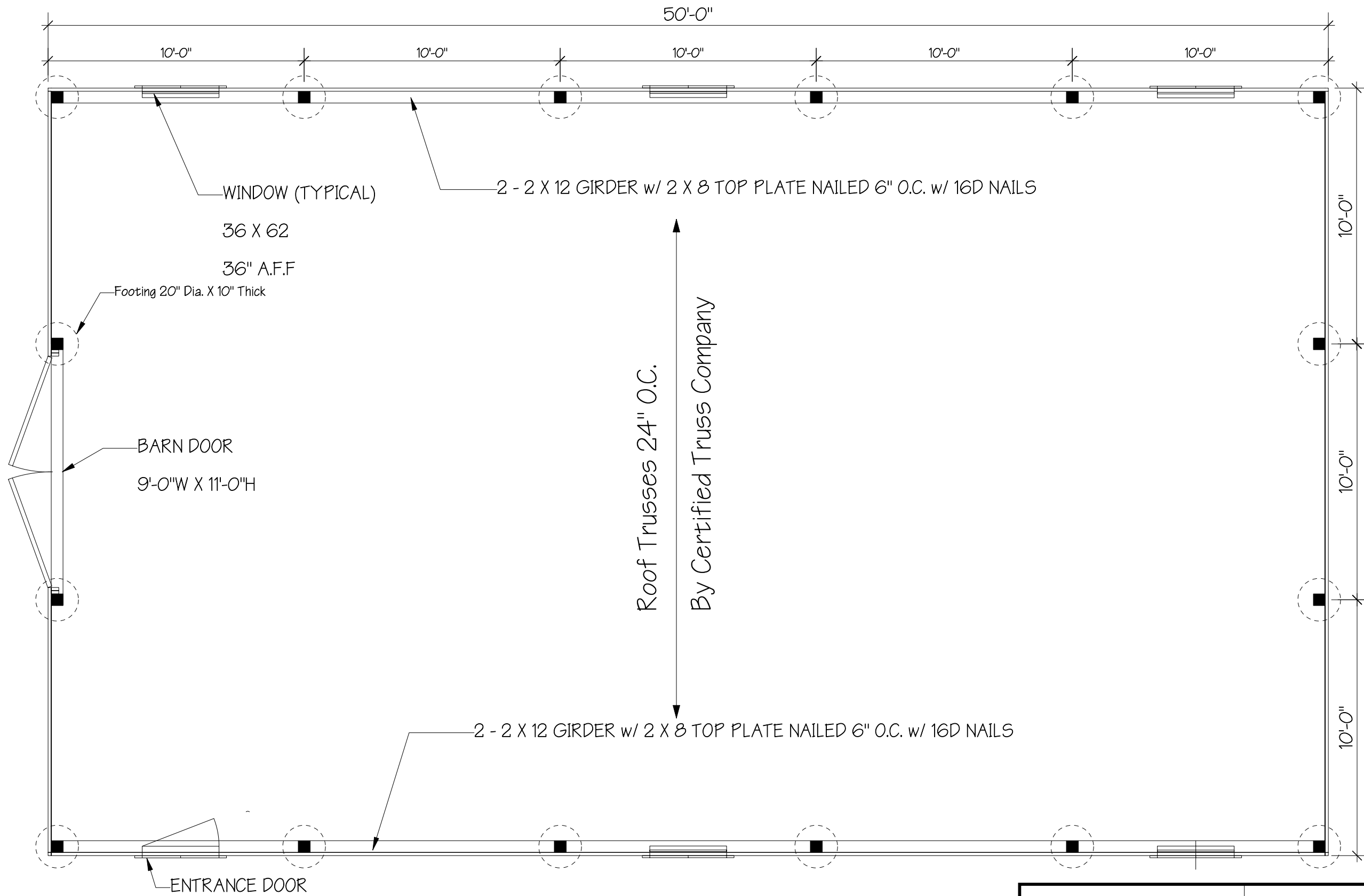
2 Floor Plan Scale: 1/4" = 1'-0"
