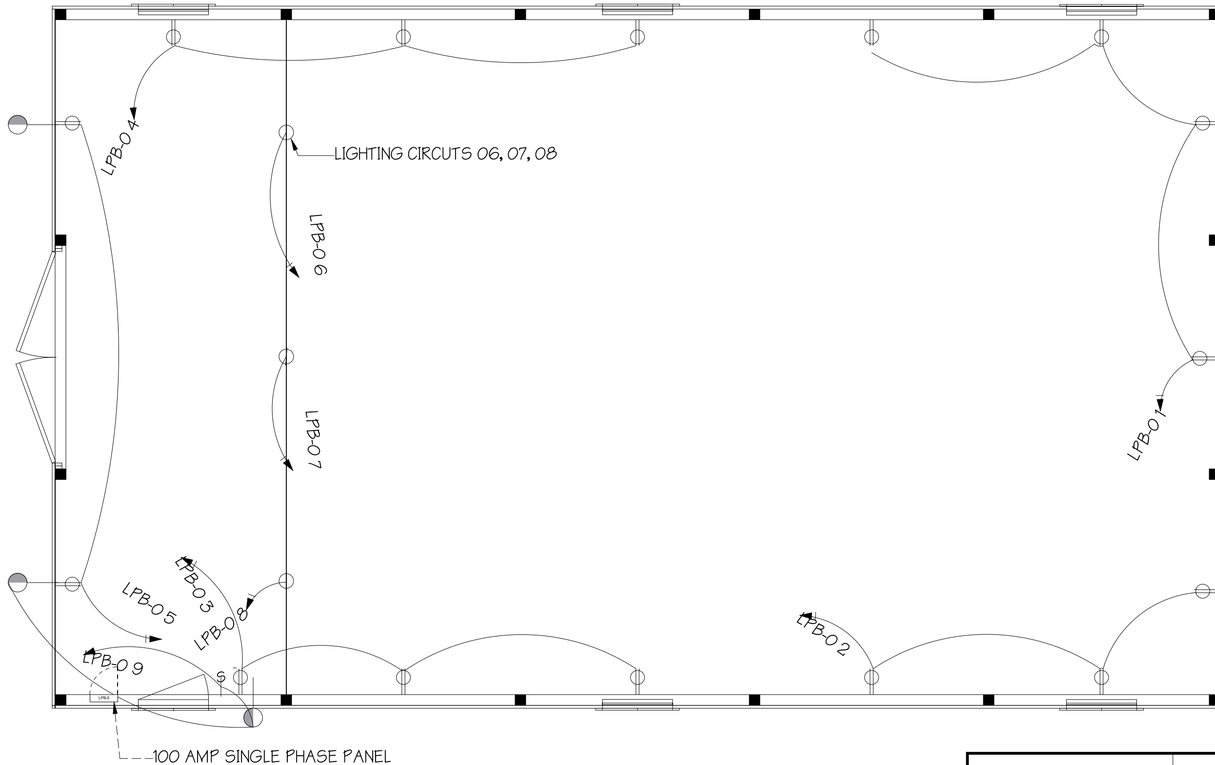
6 Electrical Plan Scale: 1/4" = 1'-0"
