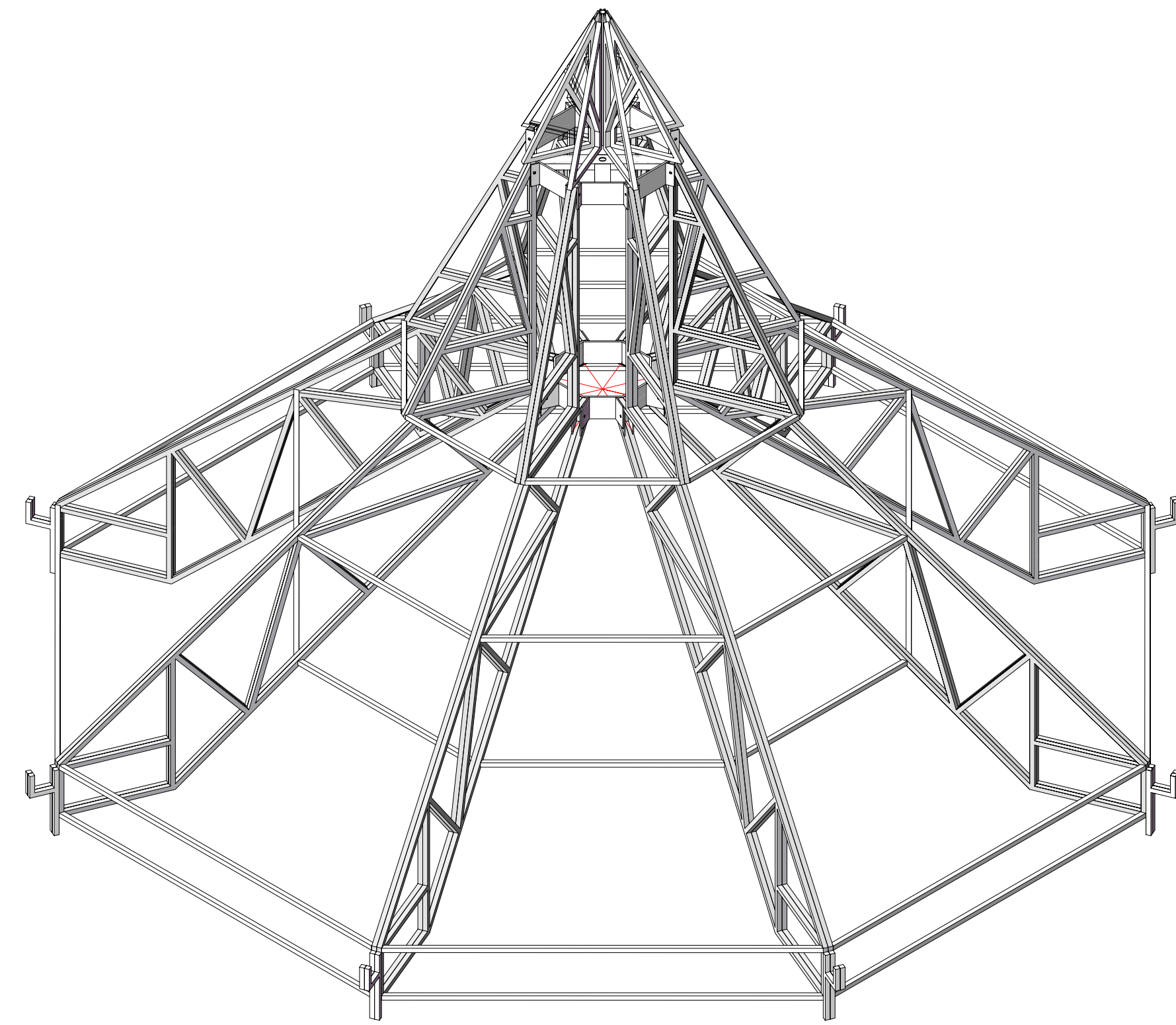
SANTA ROOM ROOF (ENTRY ROOM ROOF SIMILAR)
